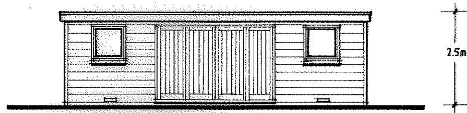
SOUTHWEST ELEVATION
